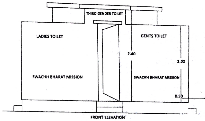
Schematic of a 2x2 community toilet
